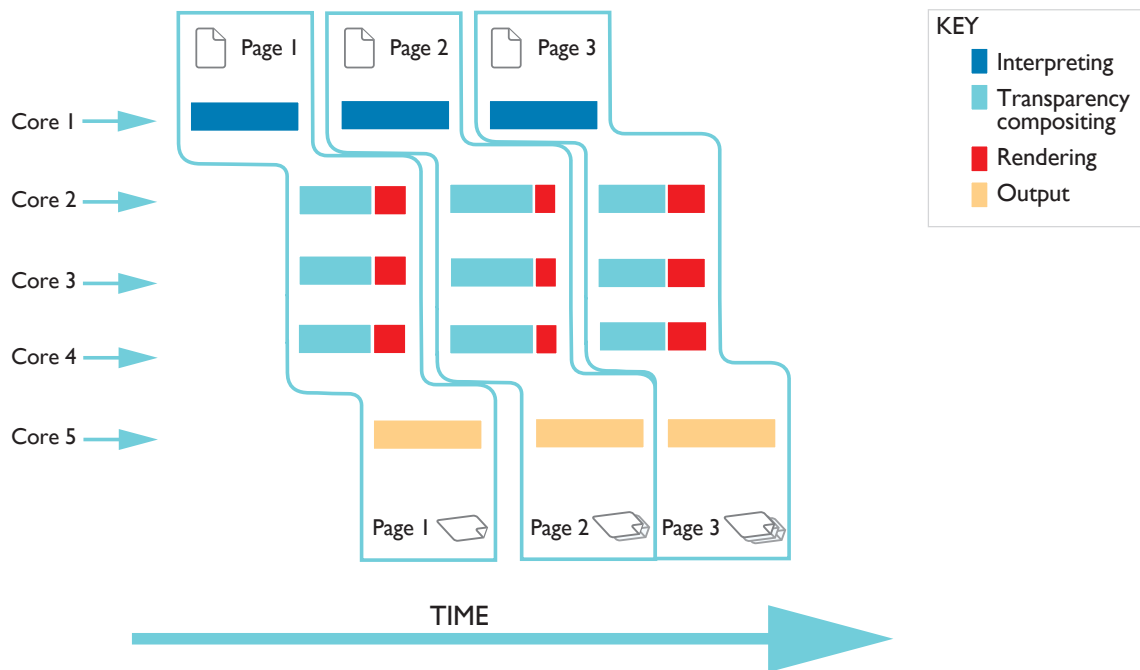
FIG 4 - Multi-threading using Harlequin Parallel Pages™. Multiple threads are used to perform the various steps of RIPing and outputting the pages of a job at once; there are no longer any periods when only a single thread is active.
