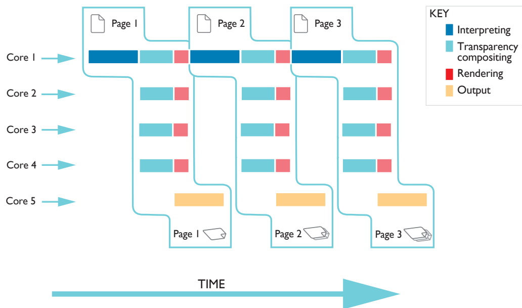
FIG 1 - Very simple Multi-threading in Harlequin Host Renderer. Multiple threads are used for transparency compositing, rendering and outputting the pages of a job at once, but interpreting introduces periods when only a single-thread is active at once.
